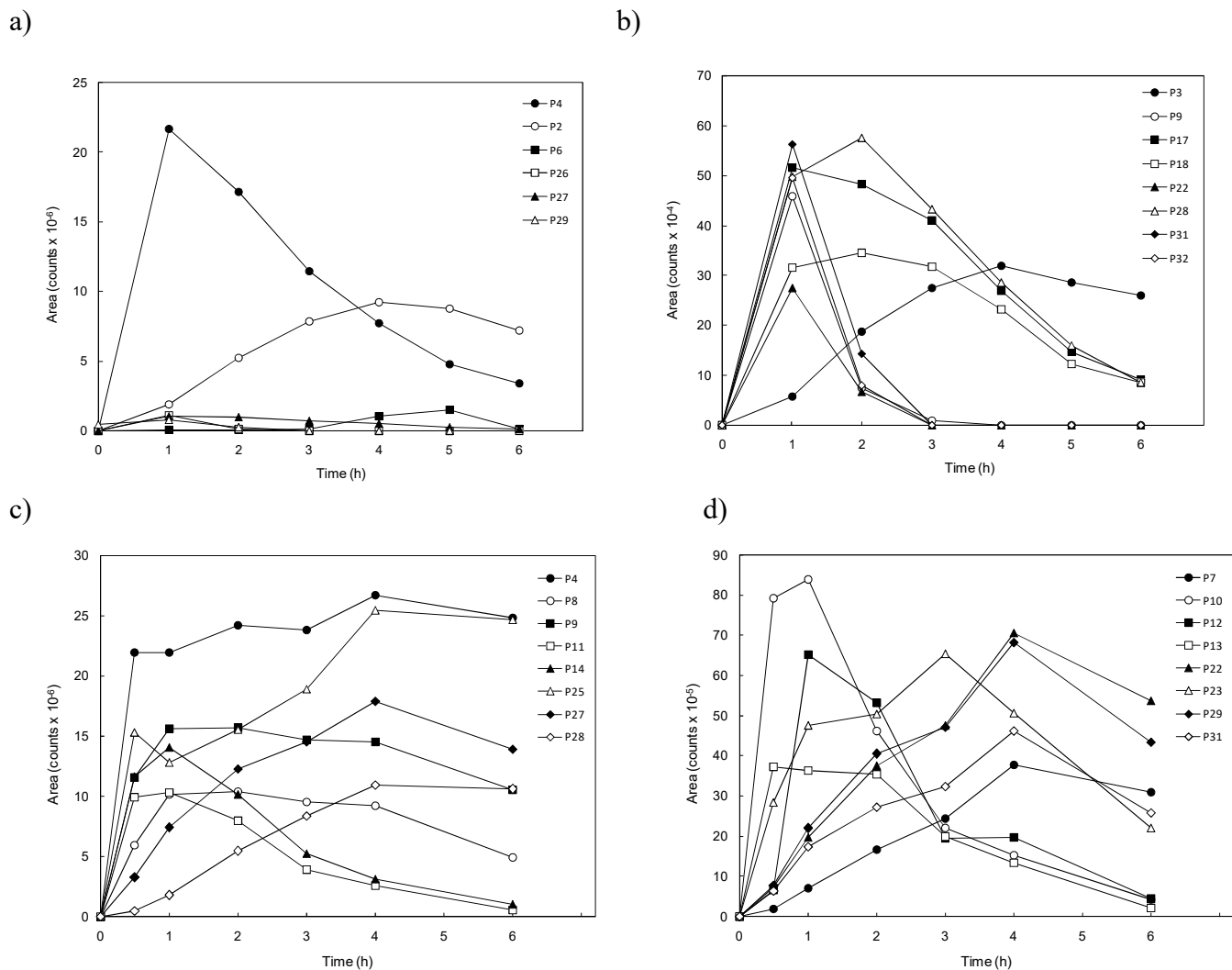
Figure 7. Chromatographic areas of the main transformation product from photocatalytic (a, b) and solar irradiation runs (c, d).
