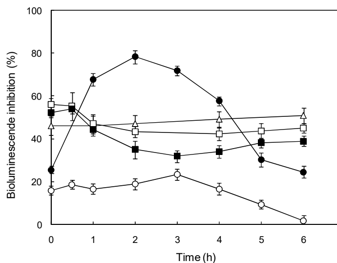
Figure 9. Bioluminescence inhibition (30 min) of V. fischeri during irradiation (○, □) and photocatalytic treatment of propranolol (●, ■, 0.14 g/L, Ce-TiO 2 0.5 % wt. cerium) in pure water (circles) and spiked wastewater (squares). (△): toxicity of non-spiked wastewater during irradiation.
