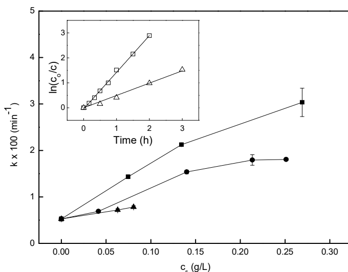
Figure 3. First-order rate constant as a function of bulk catalyst concentration for different cerium loadings: 1.0 % wt. (●), 0.5 % wt. (■) and TiO 2 without cerium (▲). Inset: fitting of the logarithmic concentration decay for pure irradiation (without catalyst, Δ) and for 75 mg/L Ce-TiO 2 , 0.5 % wt. Ce.
