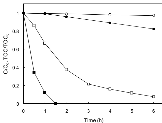
Figure 2. Evolution of propranolol (□, ■) and TOC (○, ●) during irradiation (empty symbols) and photocatalytic oxidation (0.14 g/L, Ce-TiO 2 0.5 % wt. cerium, filled symbols).
