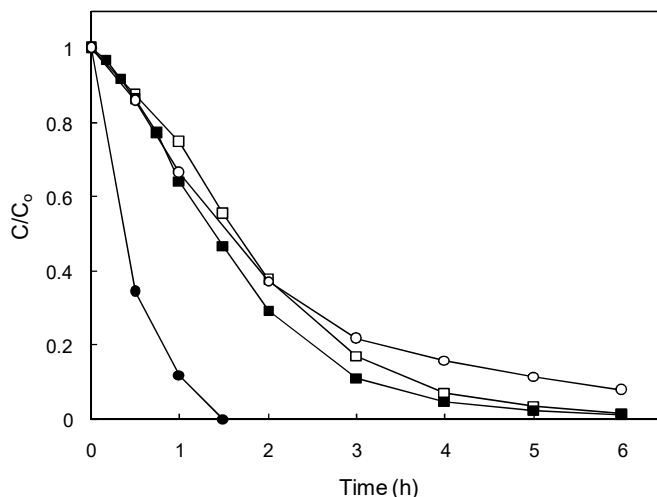
Figure 5. Propranolol depletion for irradiation ( \square ) and photocatalytic ( \blacksquare , 0.14 g/L, Ce-TiO 2 0.5 % wt. Ce) runs in spiked wastewater. For comparison similar runs in pure water are included ( \circ , \bullet ), filled symbols representing photocatalytic experiments.
