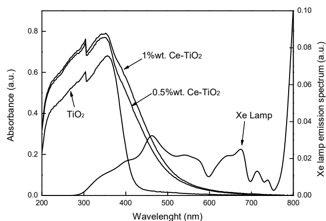
Figure 1. Catalyst absorbance for different cerium content: (1) 1.0 %, (2) 0.5 %, (3) 0 % (TiO 2 ) and lamp emission spectrum.
