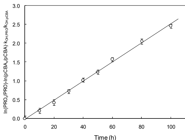
Figure 4. Fitting of competitive kinetics (Eq. 12) for the simultaneous treatment of propranolol and pCBA with 0.14 mg/L Ce-TiO 2 , 0.5 % wt. Ce.
