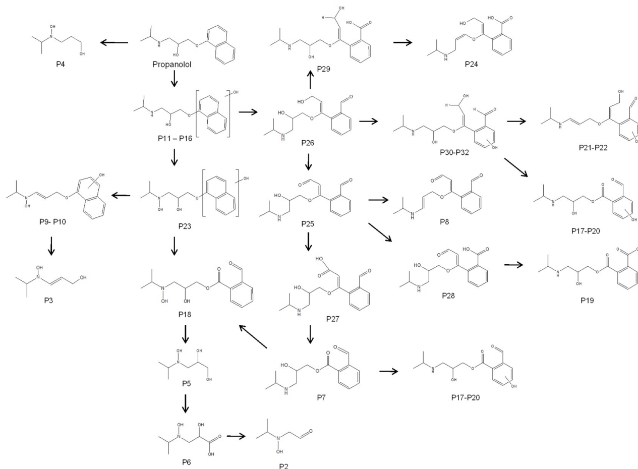
Figure 6. Proposed degradation pathway for propranolol.
